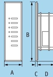
Architrave Door Jamb Control-Narrow (GRX-4S-DN) Mounts directly in door jamb. (2)
